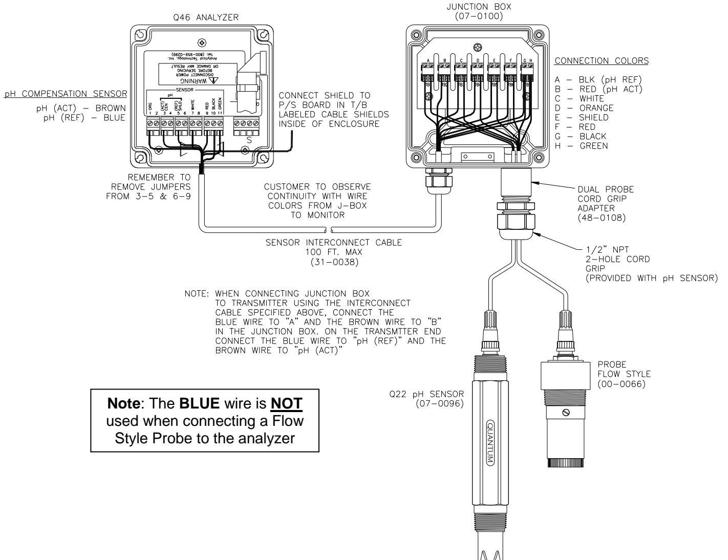
Figure 19 - Junction Box Wiring w/Optional pH Comp.
