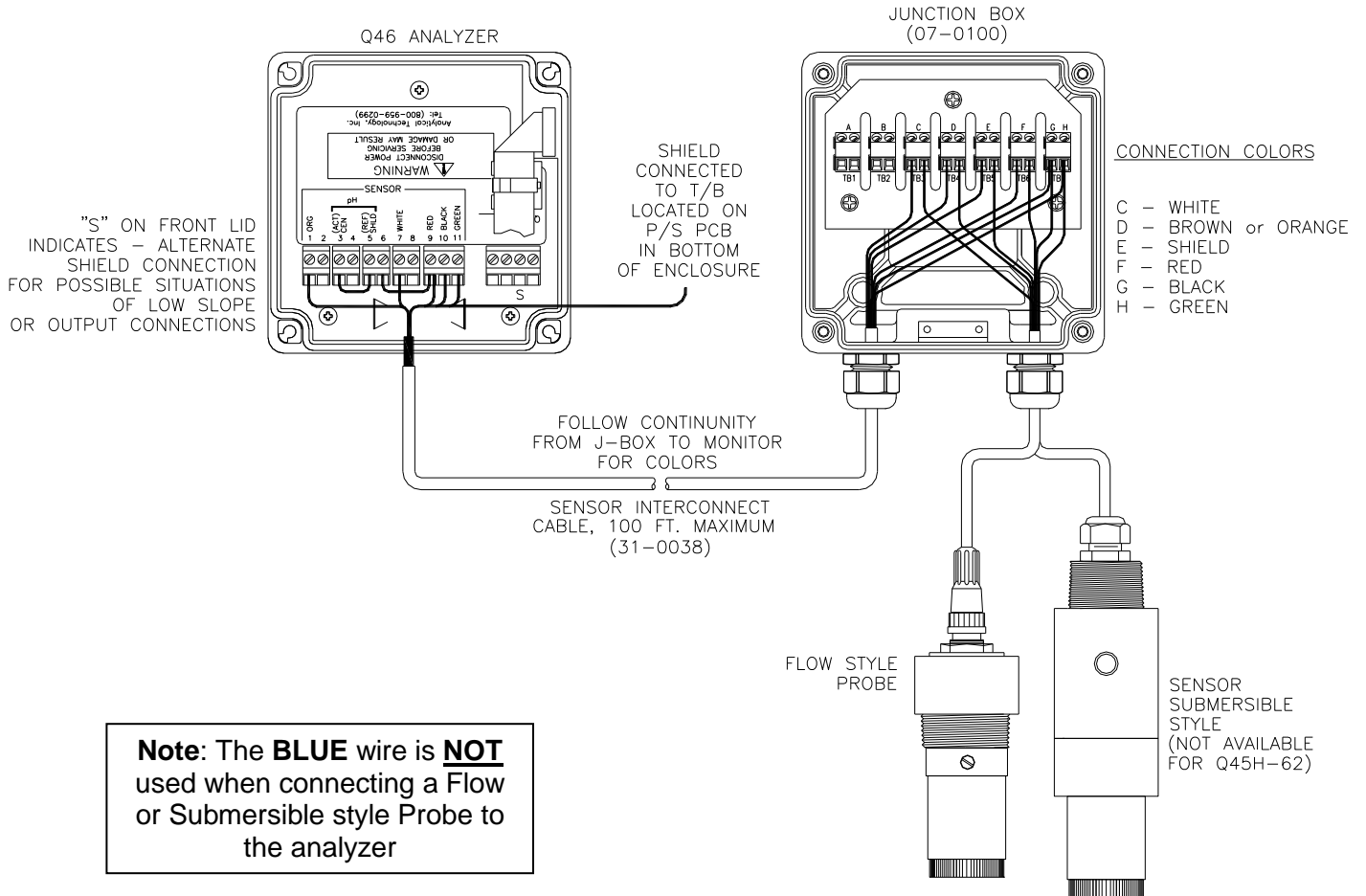
Figure 18 - Junction Box Interconnect Wiring
