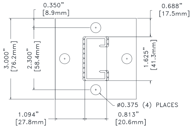
(2) GUARDRAIL BRACKET
