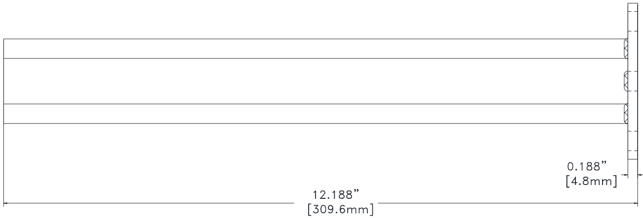
(2) GUARDRAIL BRACKET
