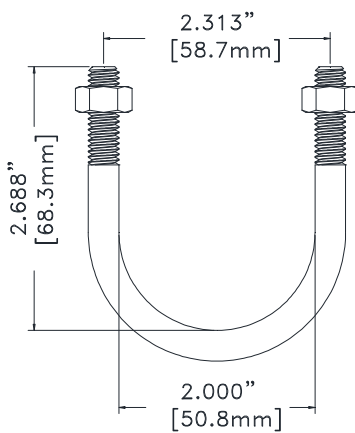
(2) U-BOLT, 5/16 - 18
