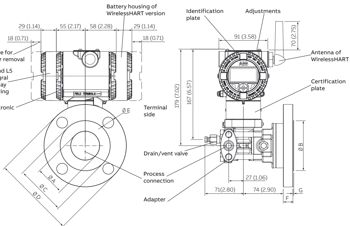
Figure 8 Transmitter with barrel housing - flange mounted version
