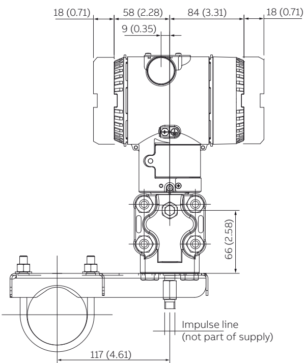
Figure 7 Transmitter with vertical flanges on bracket for vertical or horizontal 60 mm. (2 in.) pipe mounting
